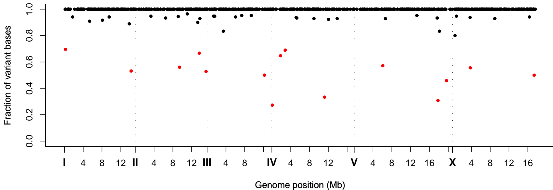
Fraction of Variant Bases at Position, Strain VC40881
