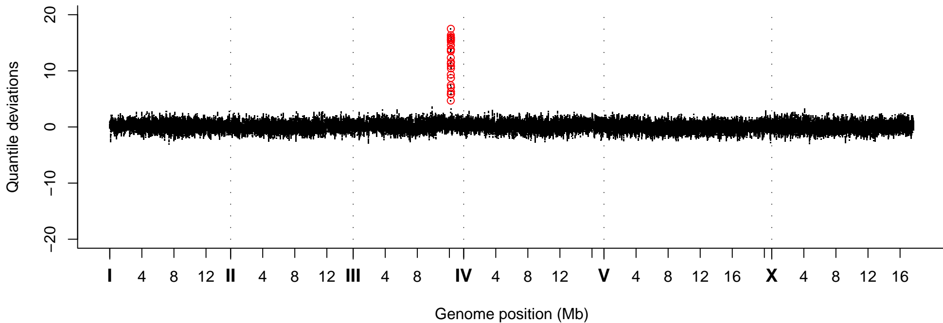
Quantile Deviations, Strain VC40881
