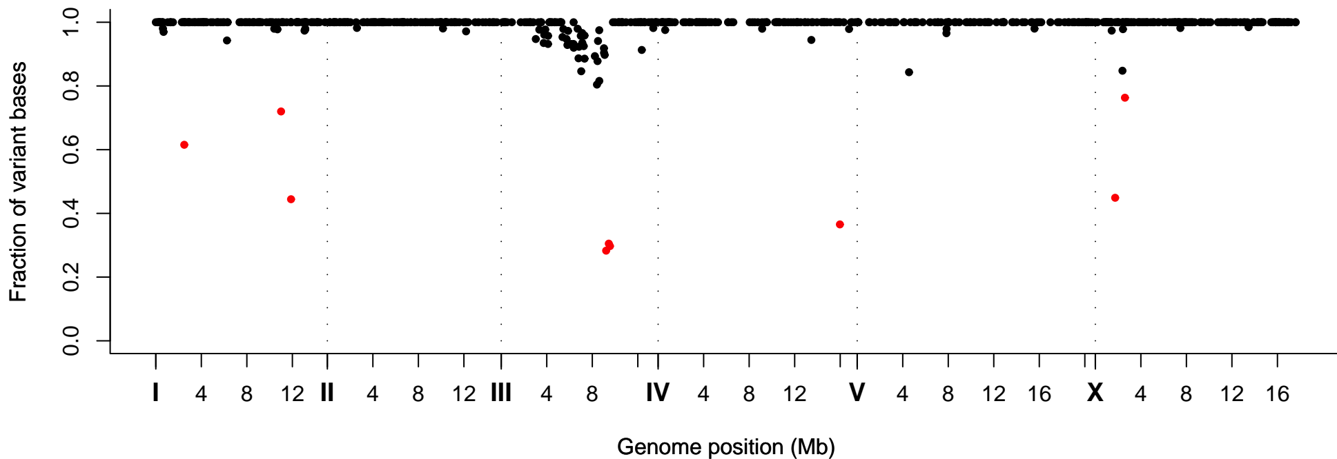
Fraction of Variant Bases at Position, Strain VC40887
