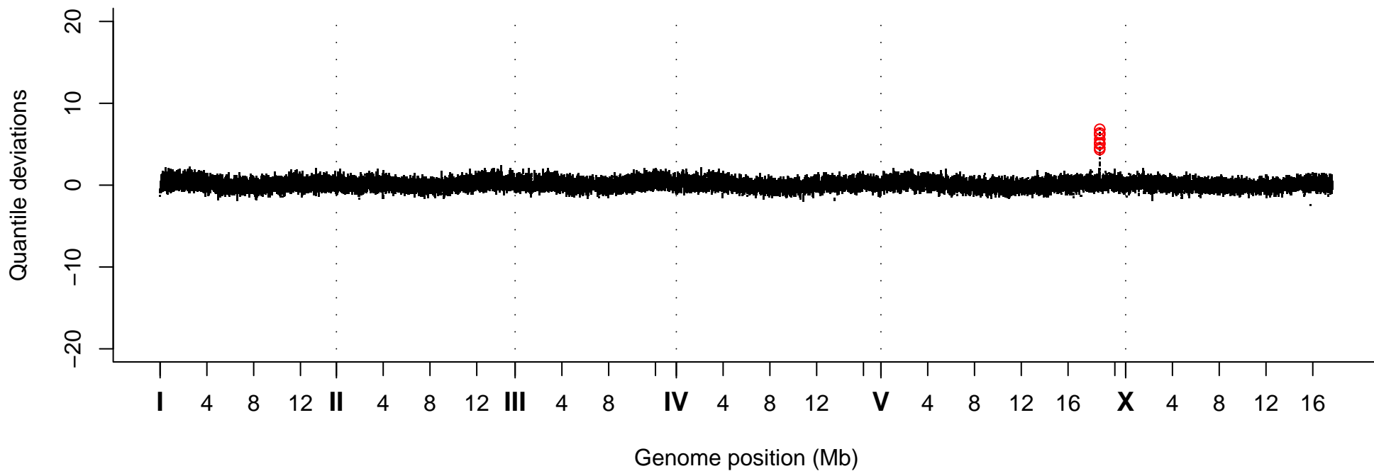
Quantile Deviations, Strain VC40887
