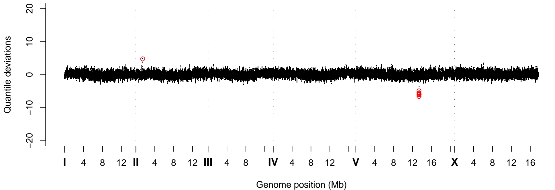
Quantile Deviations, Strain VC40893
