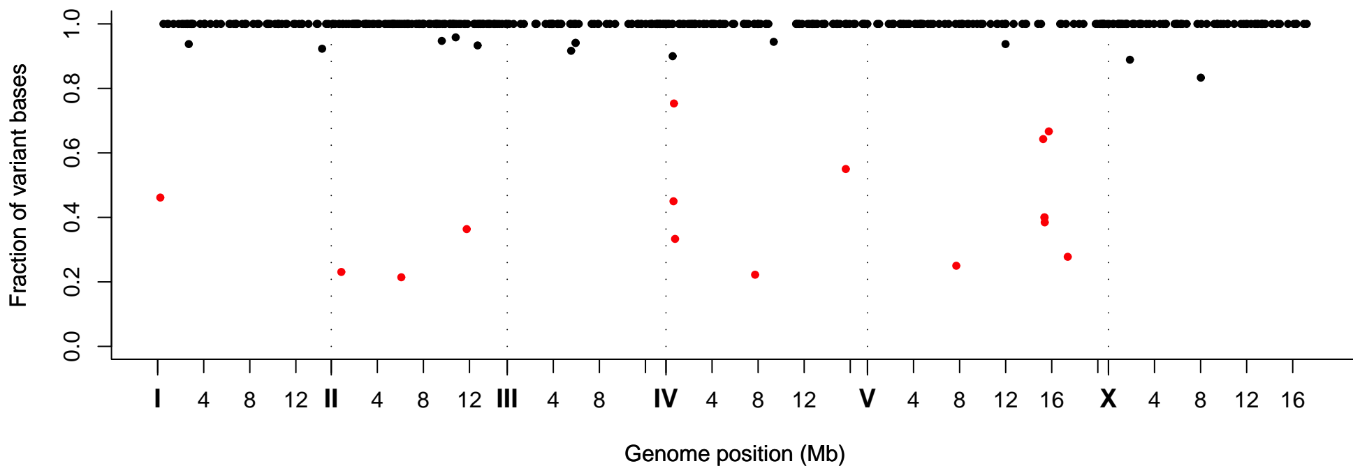
Fraction of Variant Bases at Position, Strain VC40897
