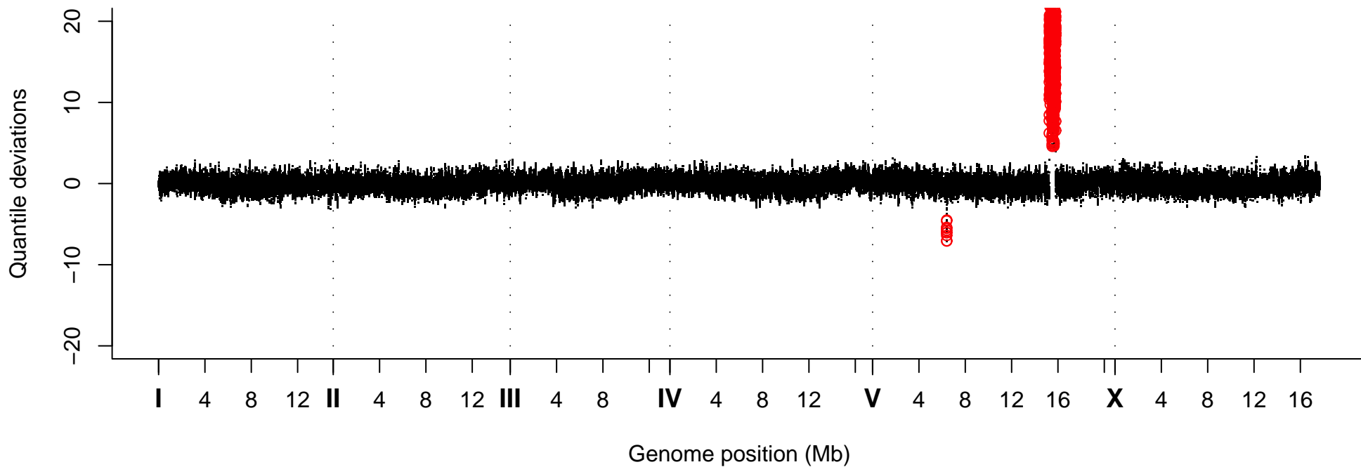
Quantile Deviations, Strain VC40897
