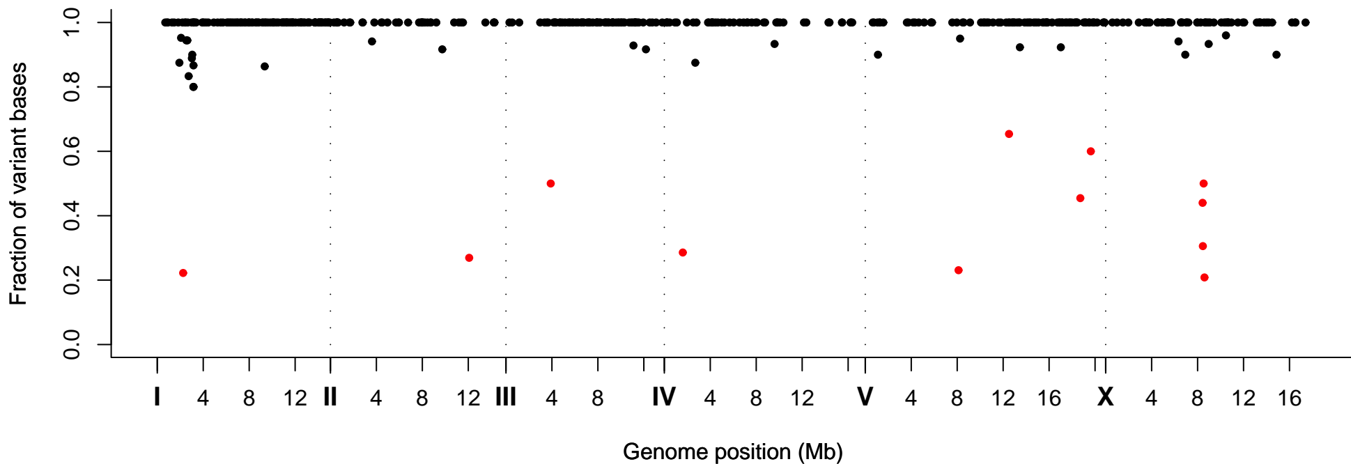
Fraction of Variant Bases at Position, Strain VC40901
