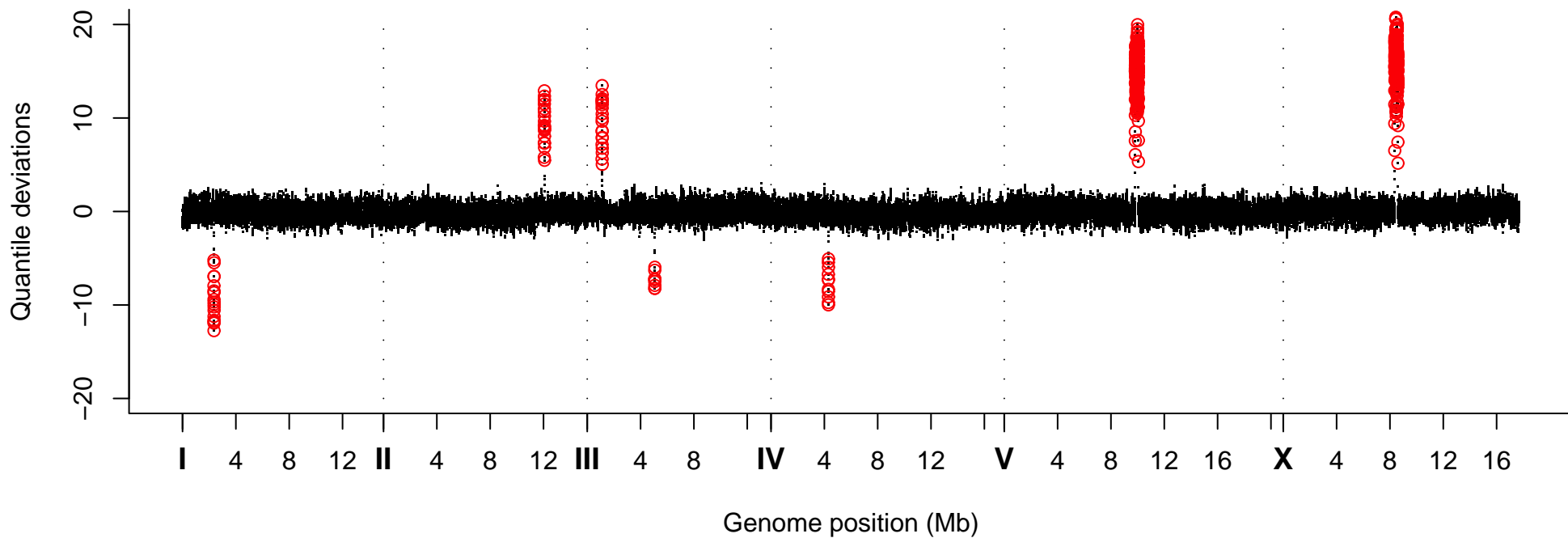
Quantile Deviations, Strain VC40901
