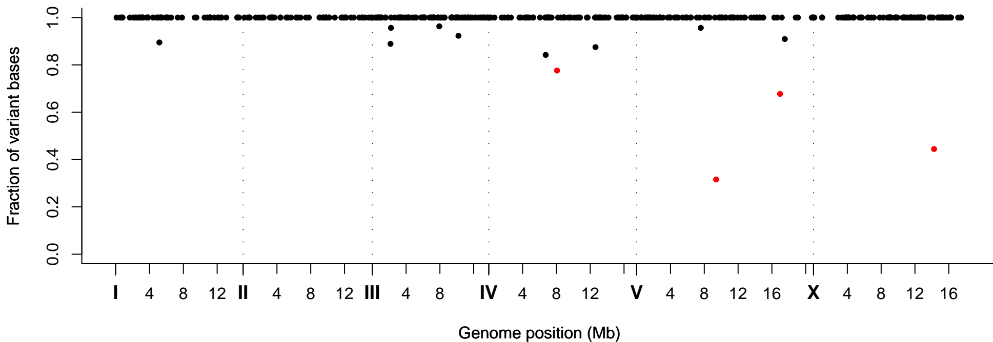
Fraction of Variant Bases at Position, Strain VC40910
