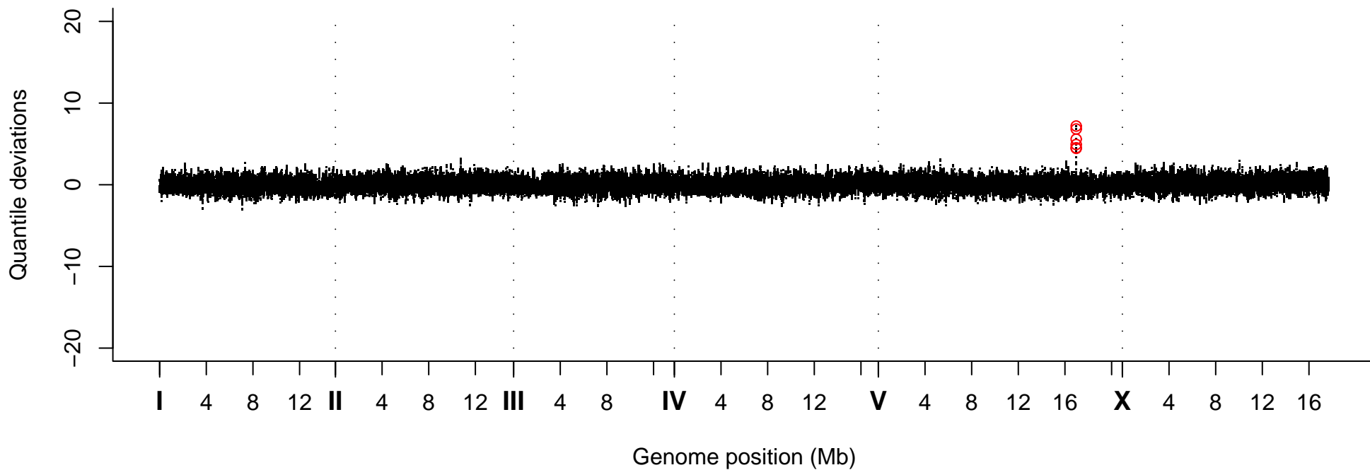
Quantile Deviations, Strain VC40910
