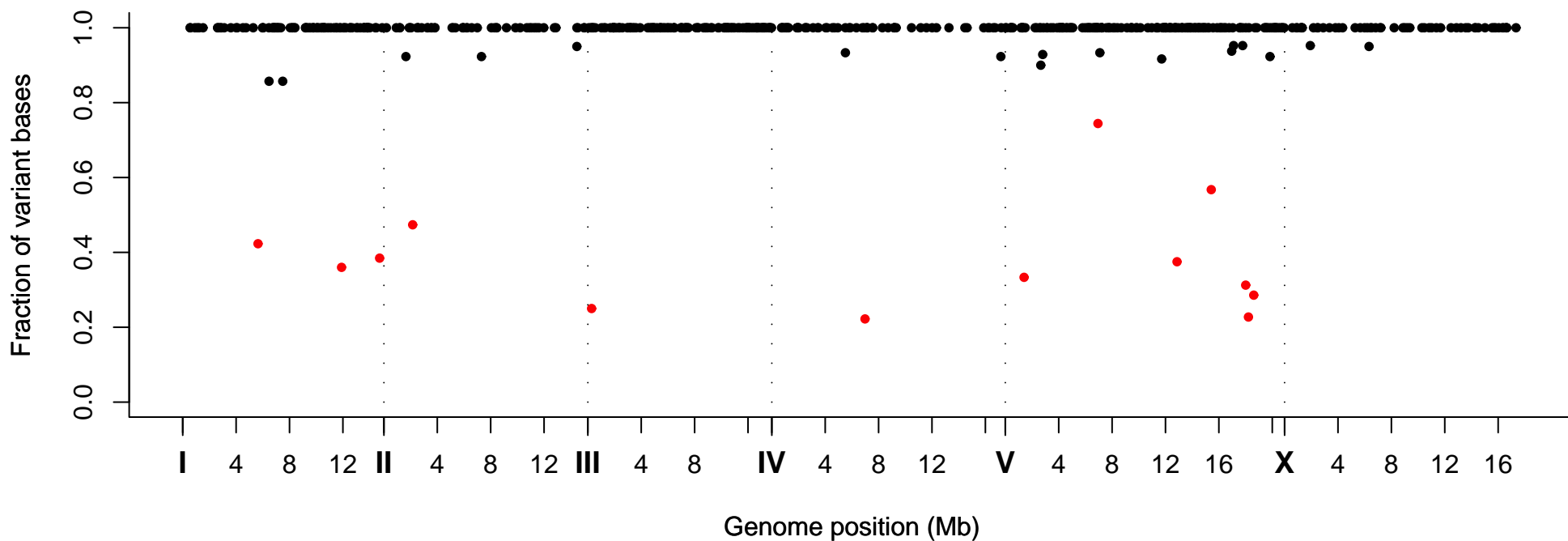
Fraction of Variant Bases at Position, Strain VC40912
