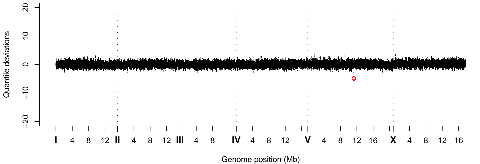
Quantile Deviations, Strain VC40912
