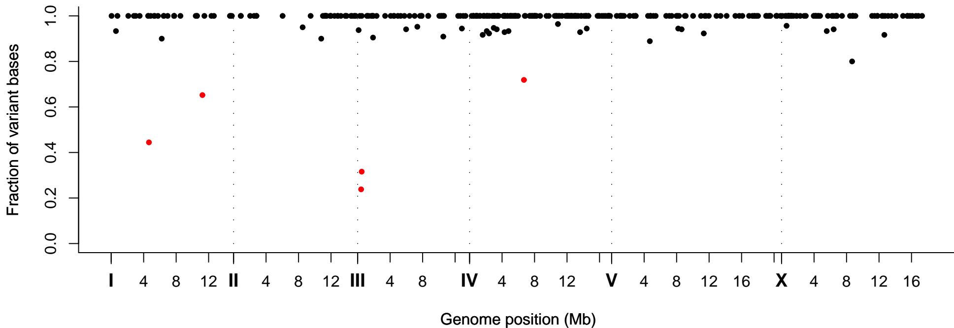
Fraction of Variant Bases at Position, Strain VC40921
