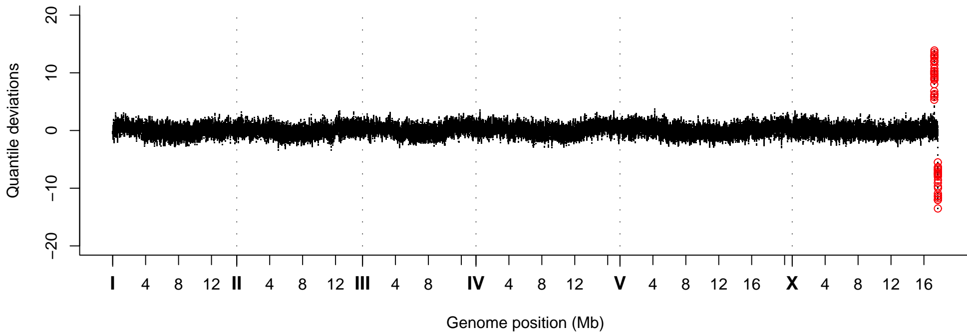
Quantile Deviations, Strain VC40921
