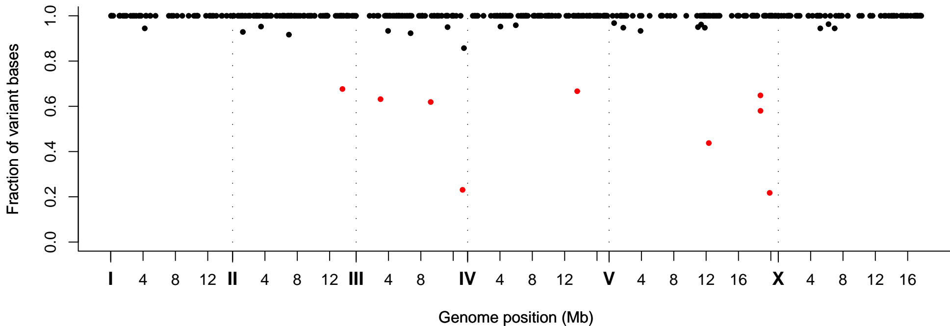
Fraction of Variant Bases at Position, Strain VC40922
