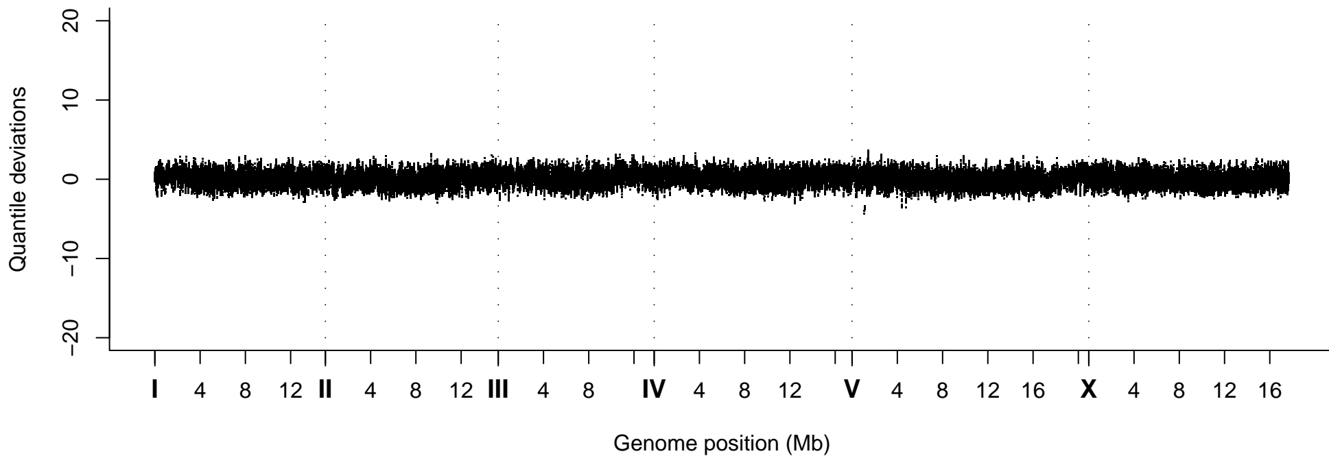
Quantile Deviations, Strain VC40922
