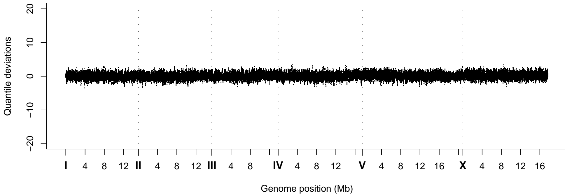
Quantile Deviations, Strain VC40924
