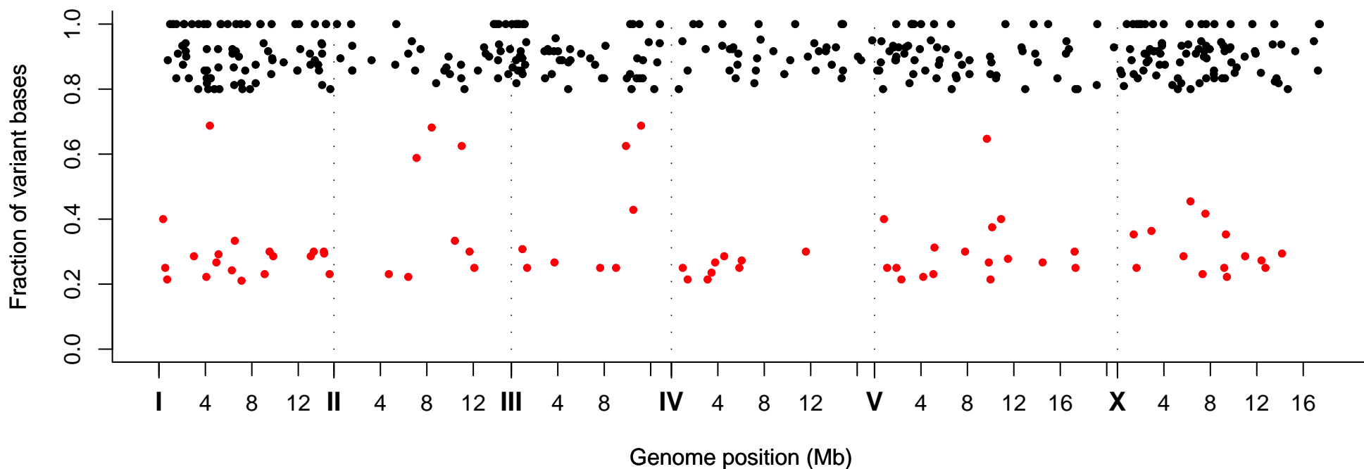
Fraction of Variant Bases at Position, Strain VC40924
