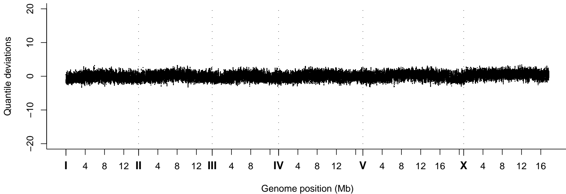
Quantile Deviations, Strain VC40932
