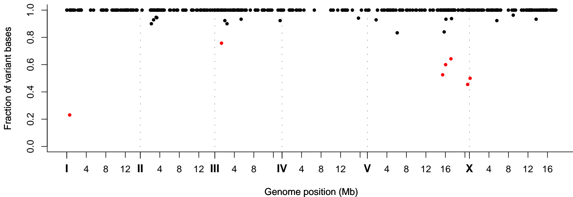
Fraction of Variant Bases at Position, Strain VC40932
