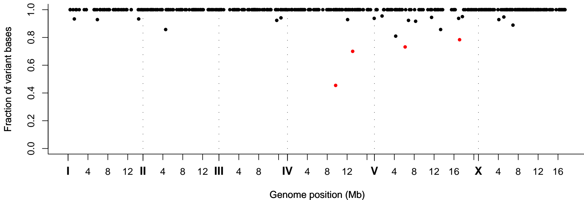
Fraction of Variant Bases at Position, Strain VC40934
