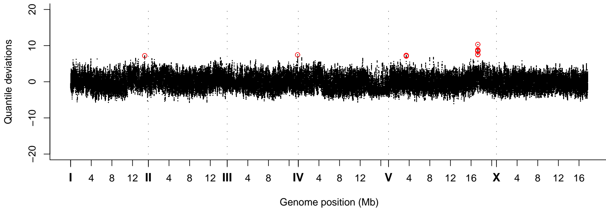
Quantile Deviations, Strain VC40936
