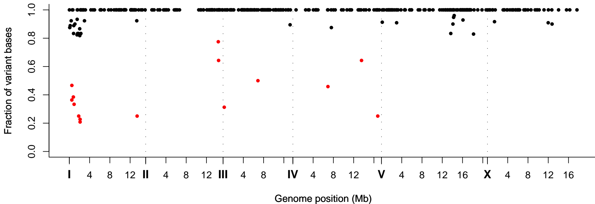
Fraction of Variant Bases at Position, Strain VC40936
