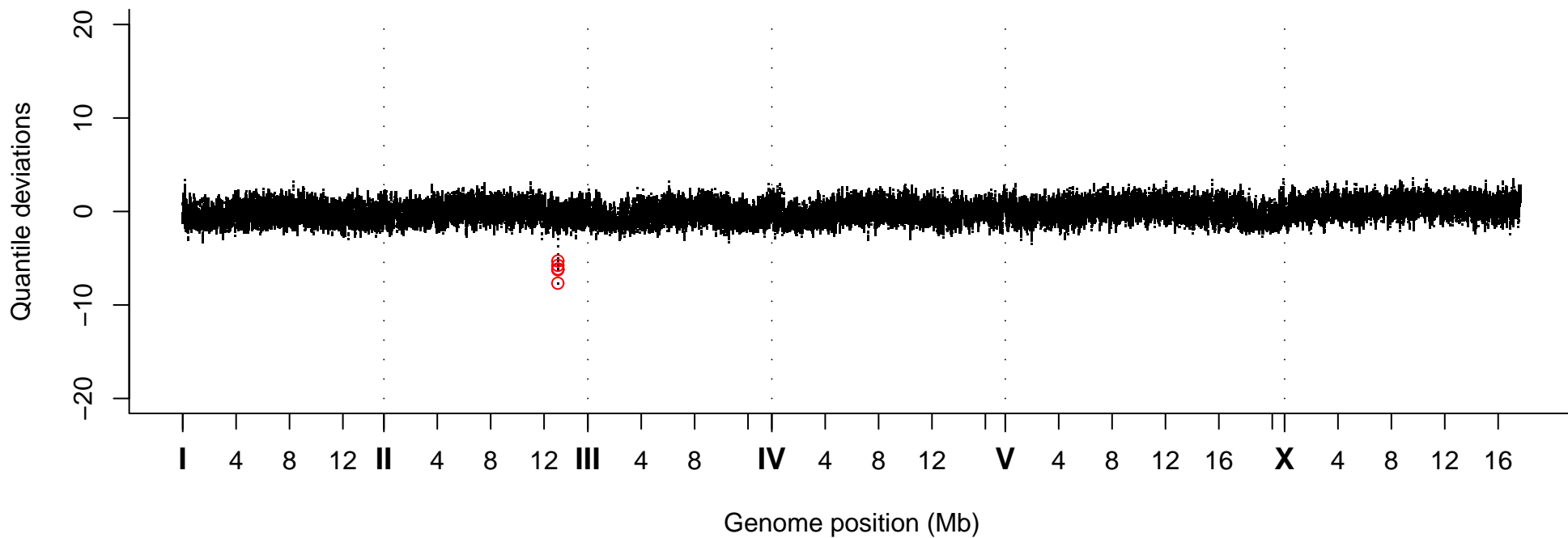
Quantile Deviations, Strain VC40937
