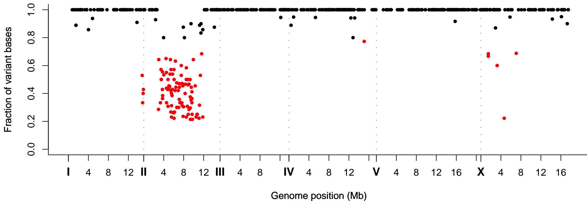
Fraction of Variant Bases at Position, Strain VC40937
