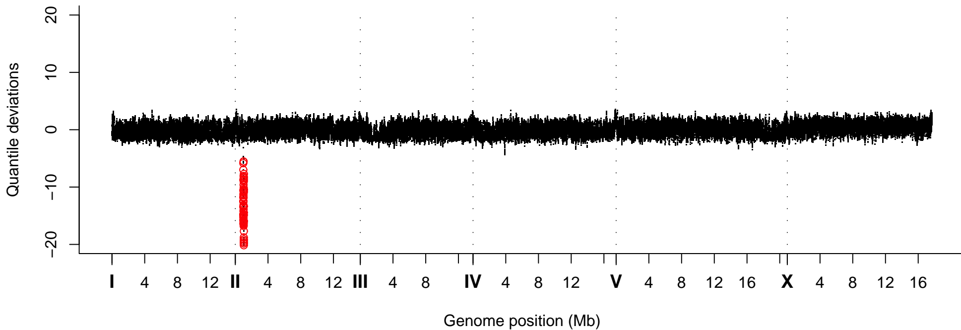
Quantile Deviations, Strain VC40948
