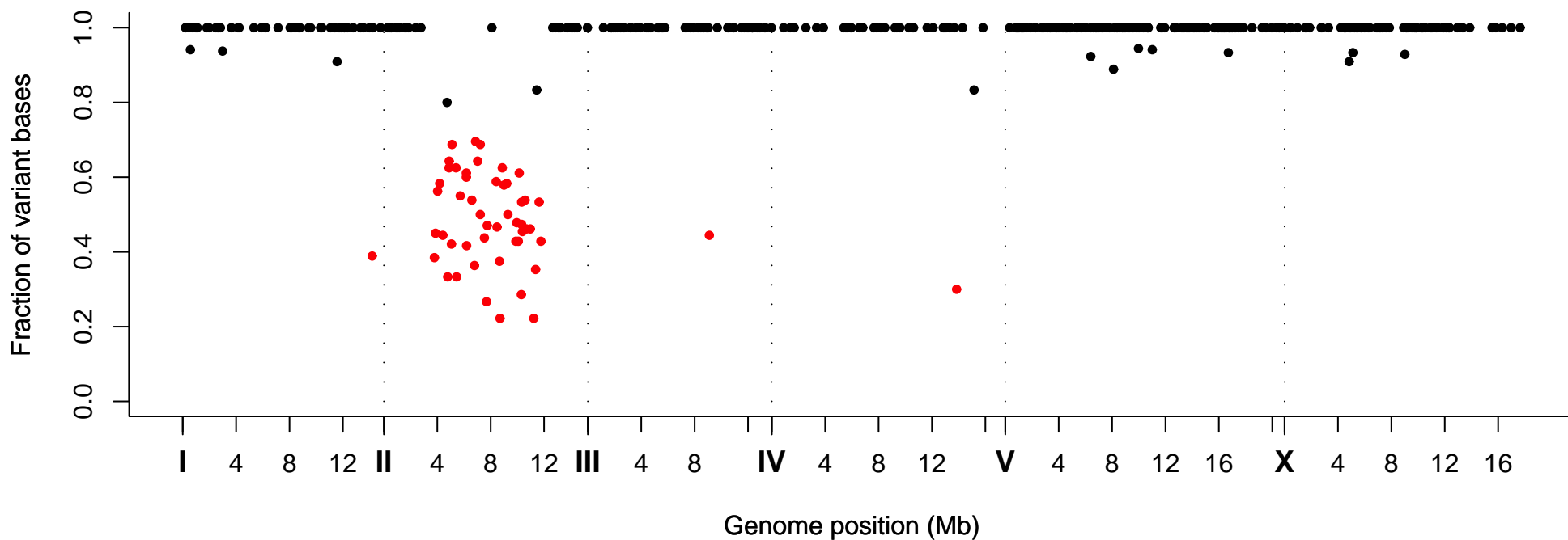
Fraction of Variant Bases at Position, Strain VC40948
