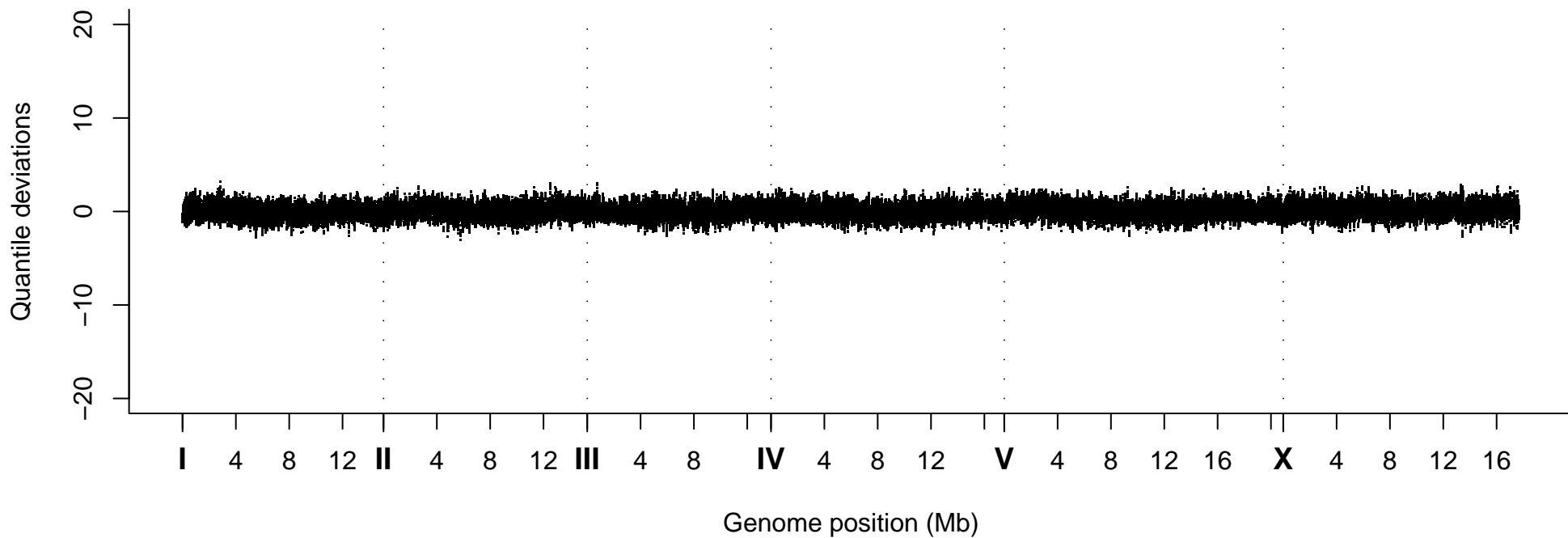
Quantile Deviations, Strain VC40955
