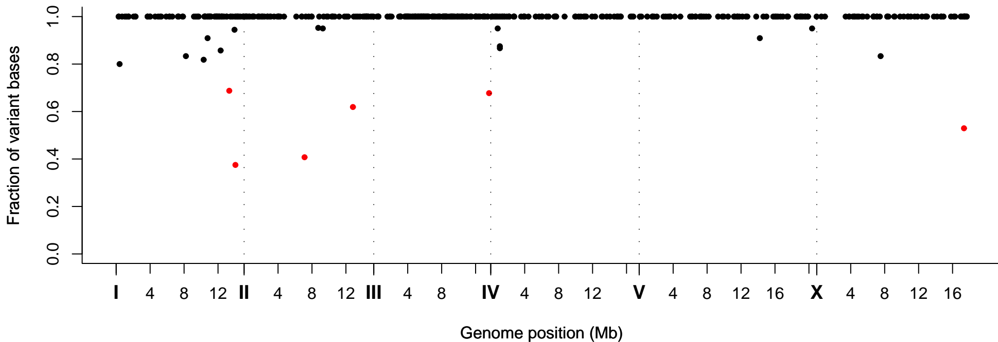
Fraction of Variant Bases at Position, Strain VC40955
