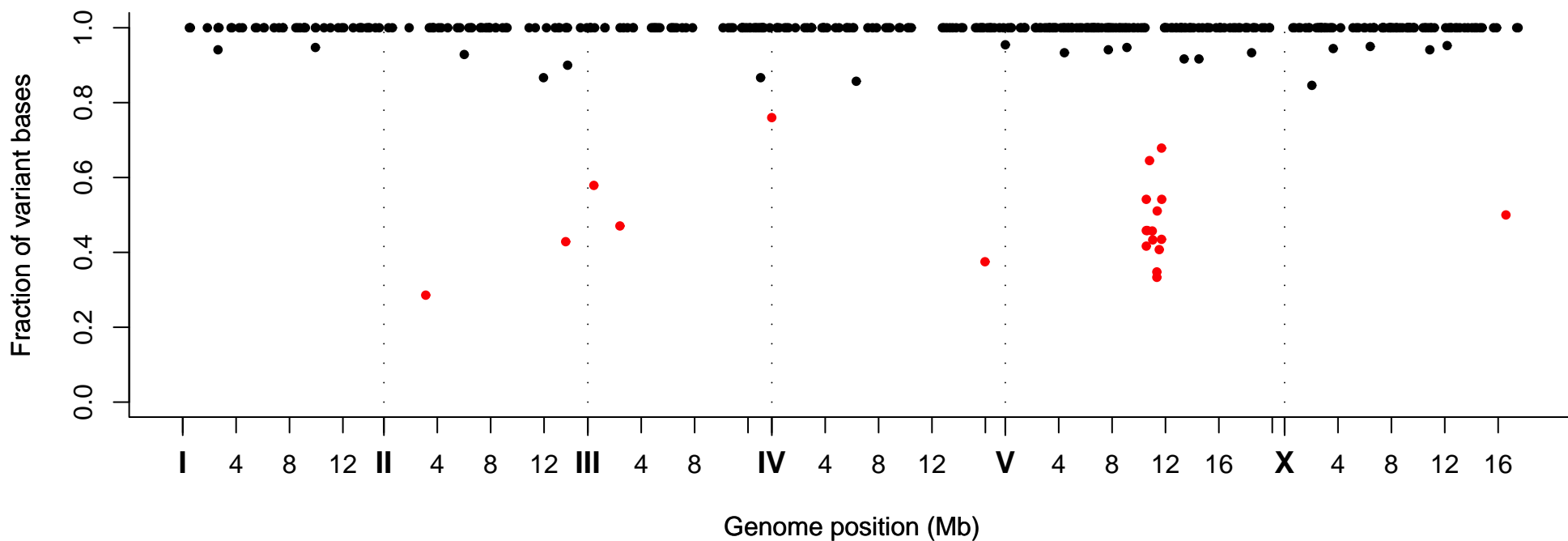
Fraction of Variant Bases at Position, Strain VC40956
