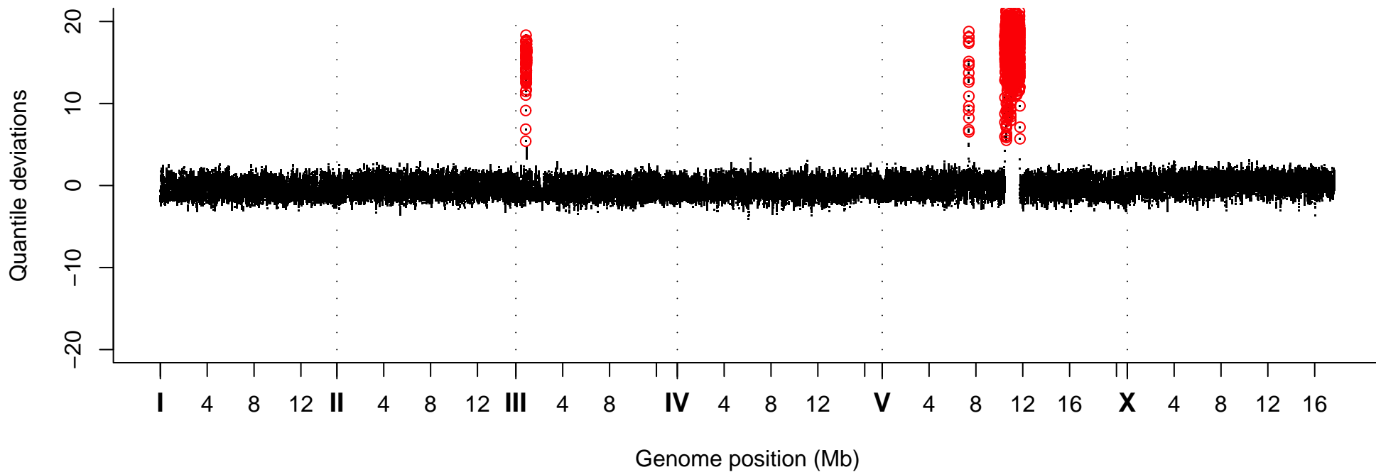
Quantile Deviations, Strain VC40956
