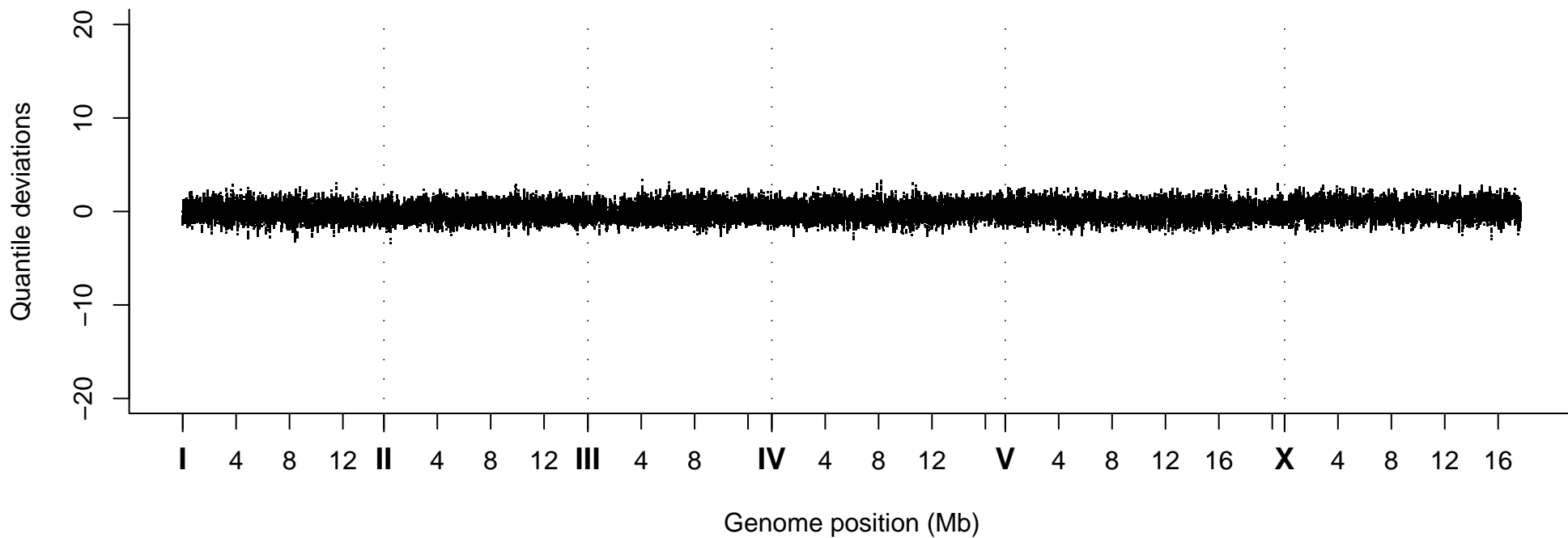
Quantile Deviations, Strain VC40960
