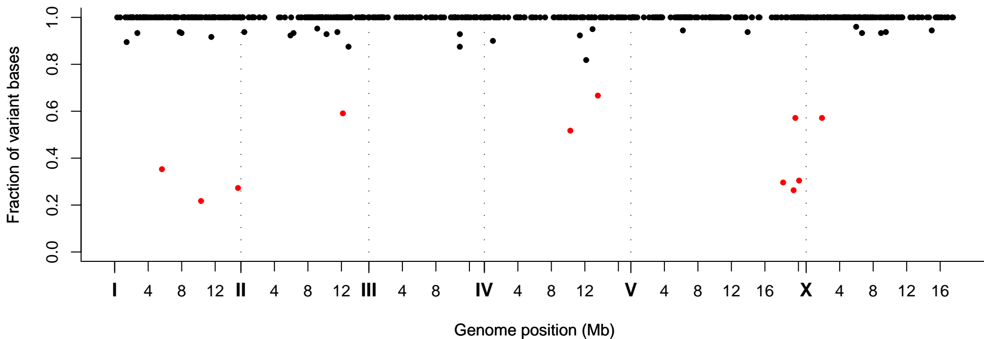
Fraction of Variant Bases at Position, Strain VC40960
