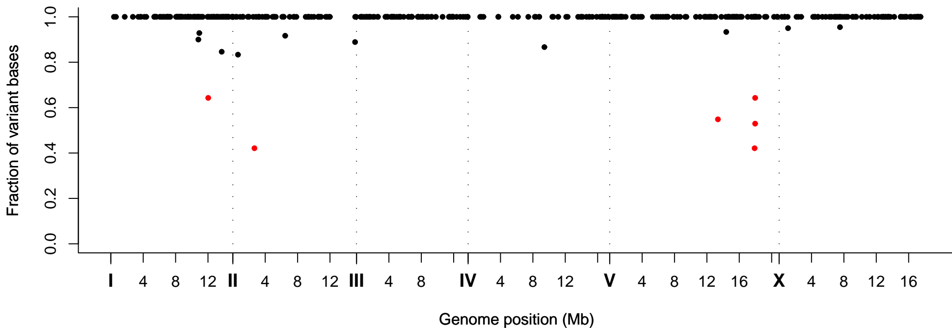
Fraction of Variant Bases at Position, Strain VC40961
