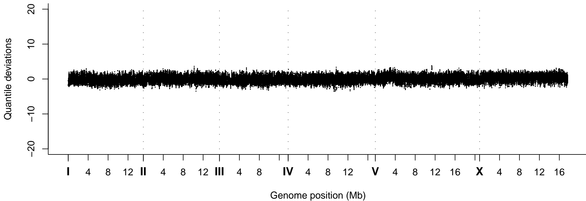
Quantile Deviations, Strain VC40961
