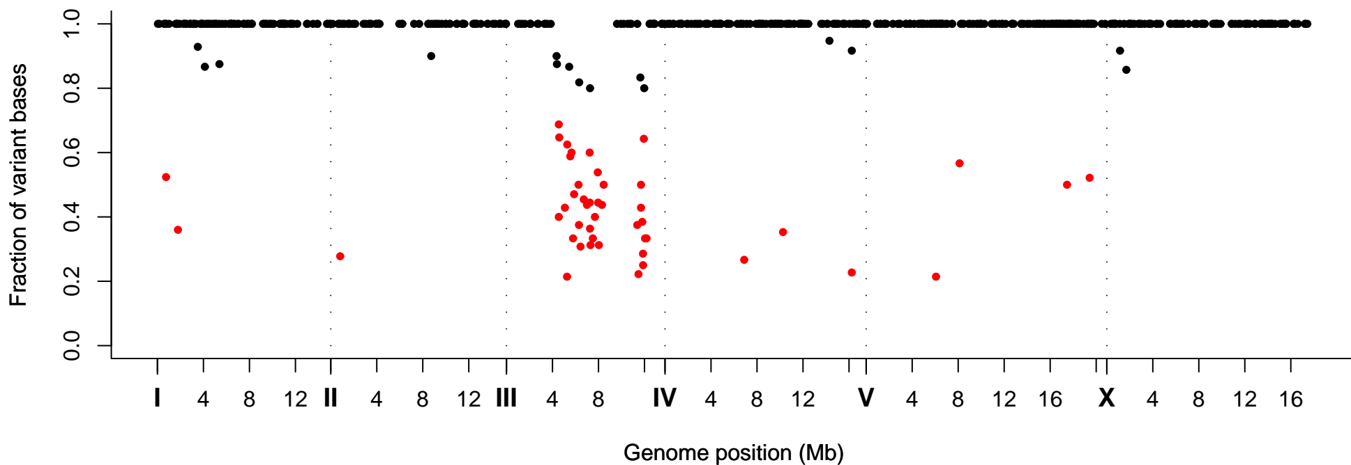
Fraction of Variant Bases at Position, Strain VC40962
