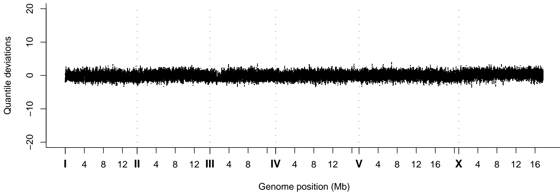
Quantile Deviations, Strain VC40962
