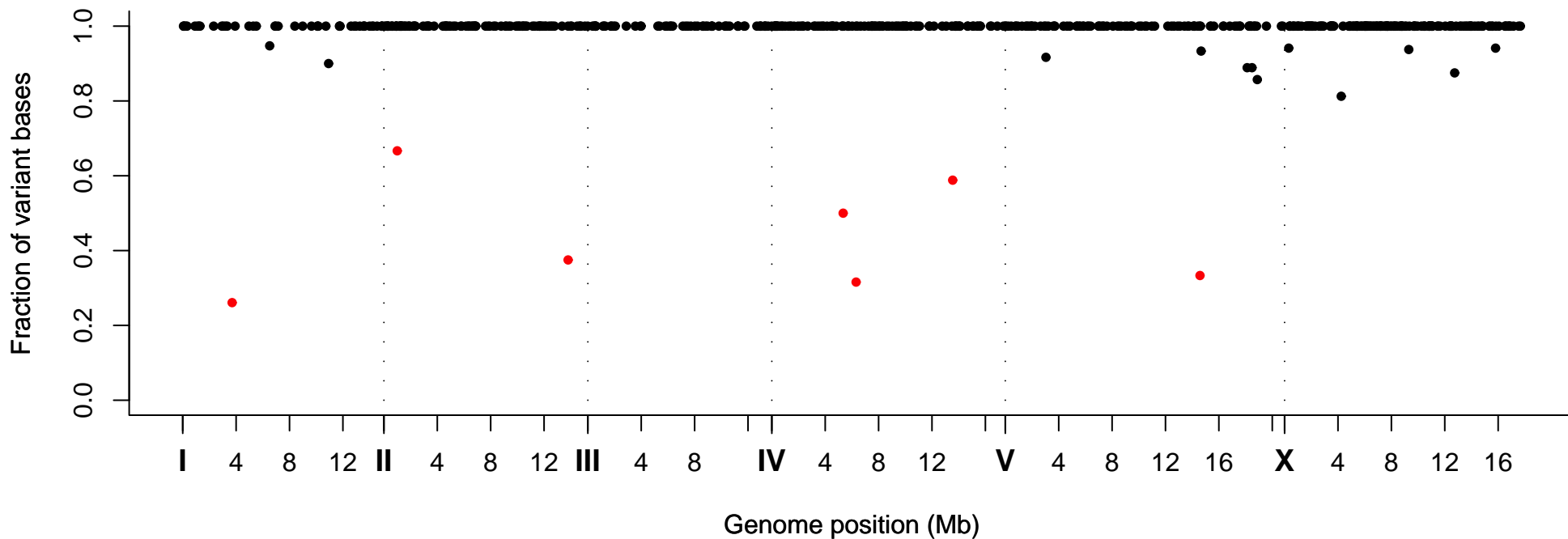
Fraction of Variant Bases at Position, Strain VC40963
