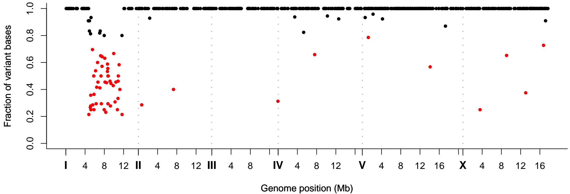
Fraction of Variant Bases at Position, Strain VC40965
