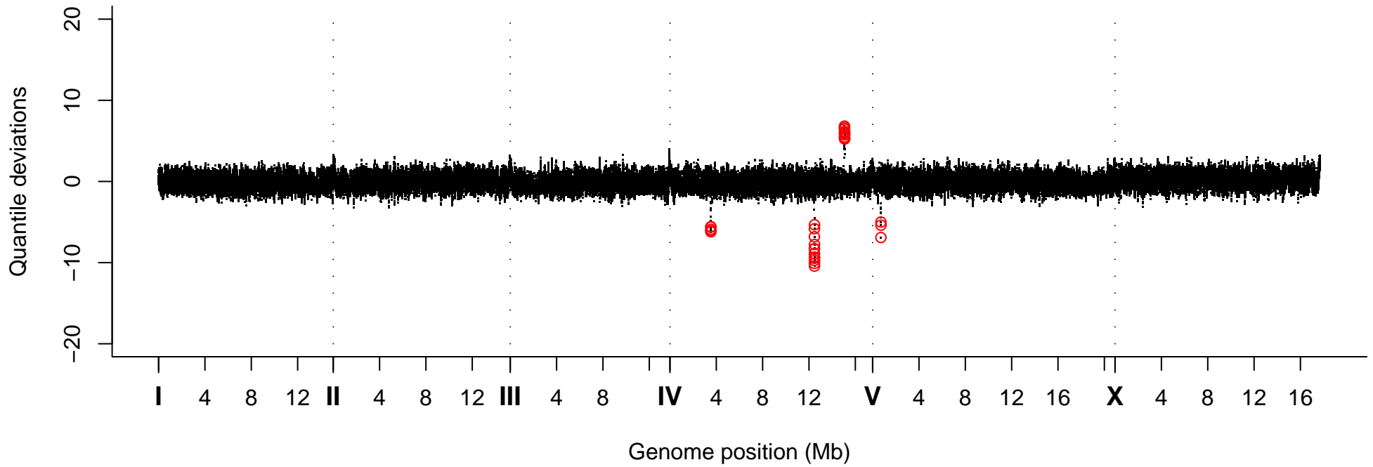
Quantile Deviations, Strain VC40965
