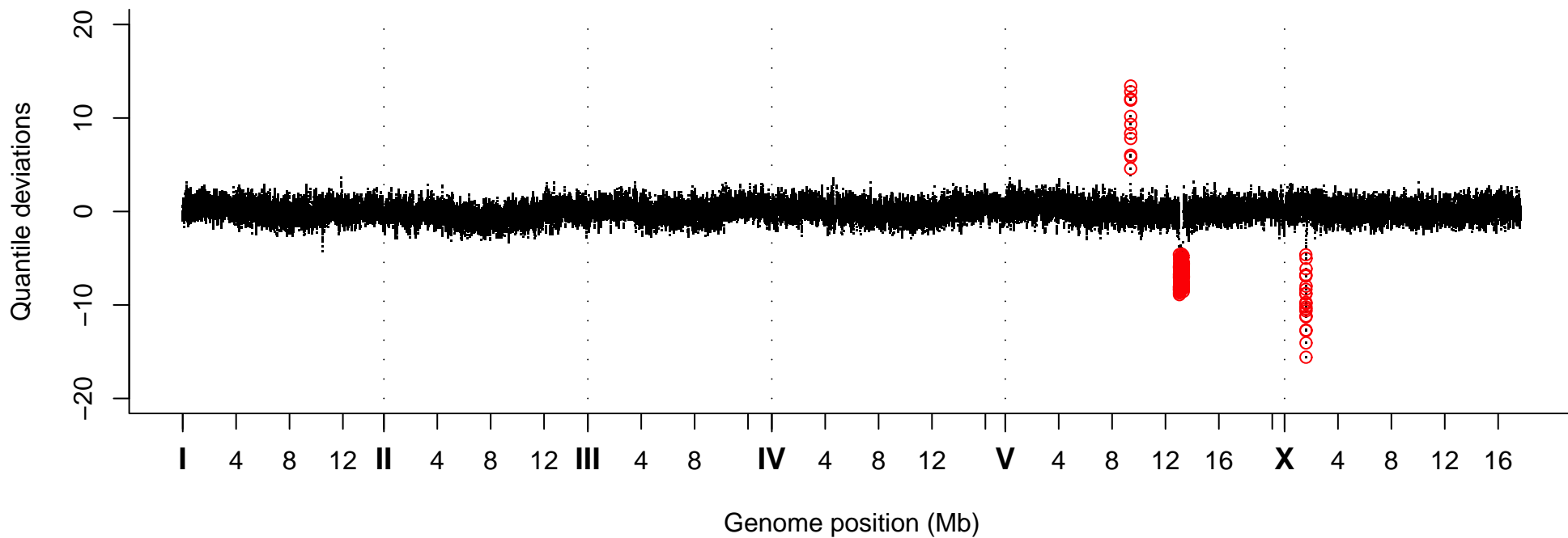
Quantile Deviations, Strain VC40971
