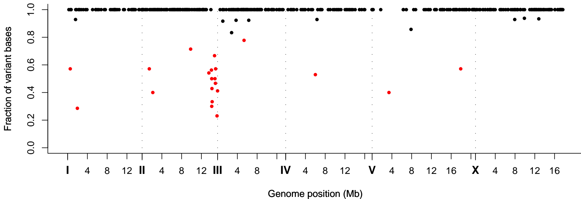
Fraction of Variant Bases at Position, Strain VC40973
