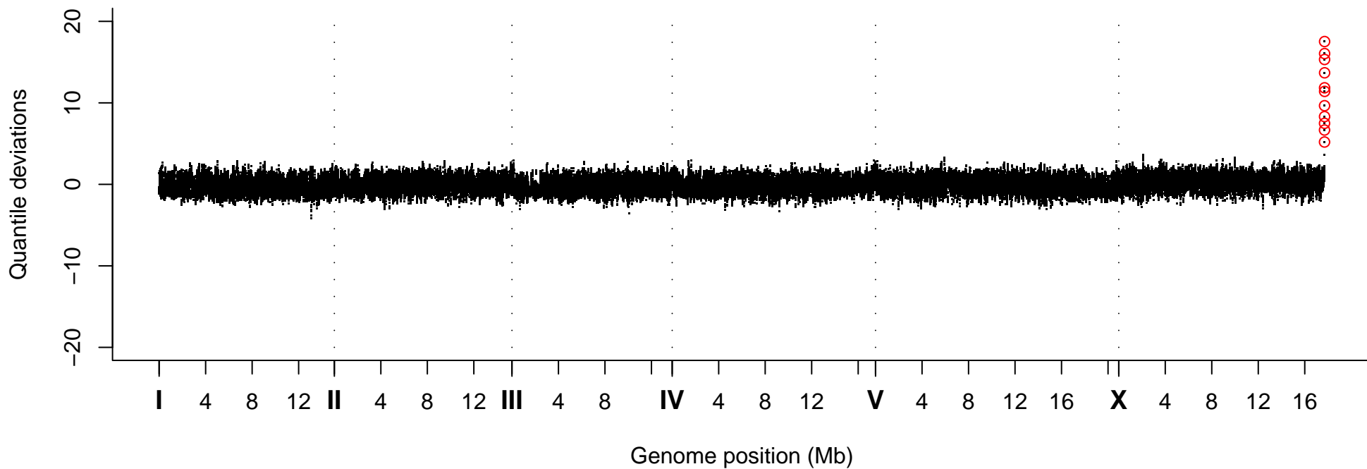
Quantile Deviations, Strain VC40973
