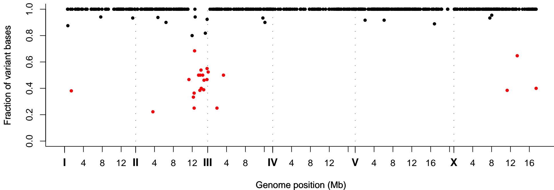
Fraction of Variant Bases at Position, Strain VC40974
