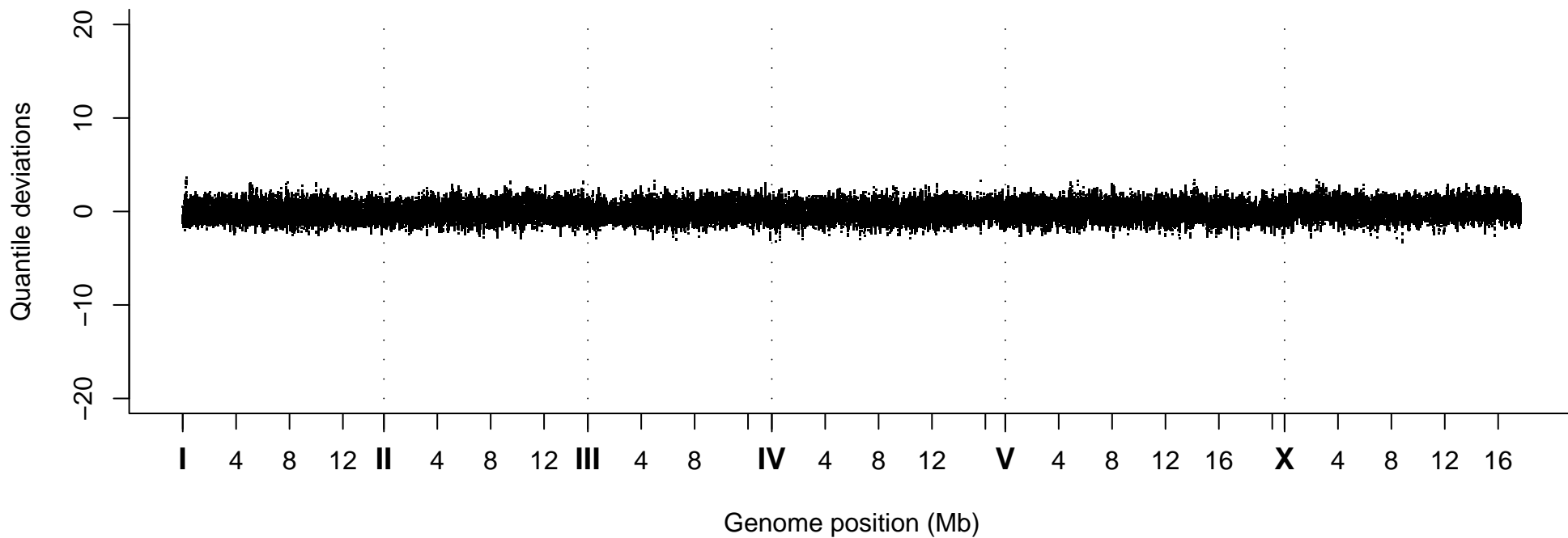
Quantile Deviations, Strain VC40974
