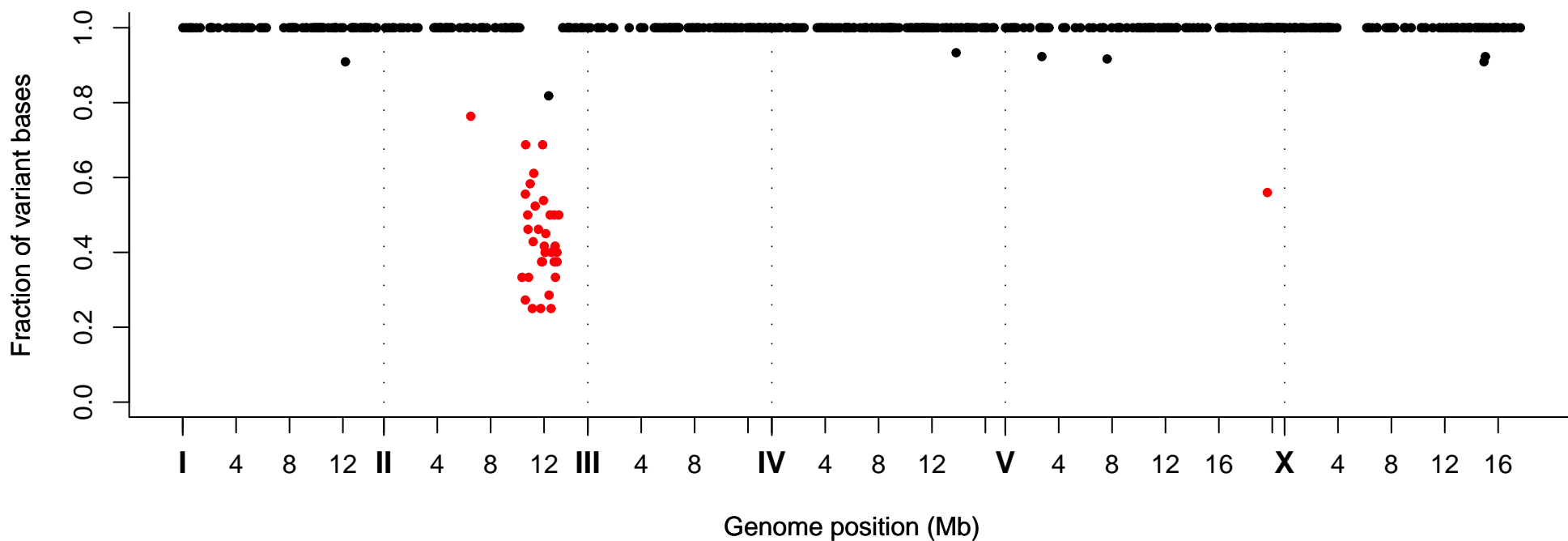
Fraction of Variant Bases at Position, Strain VC40975
