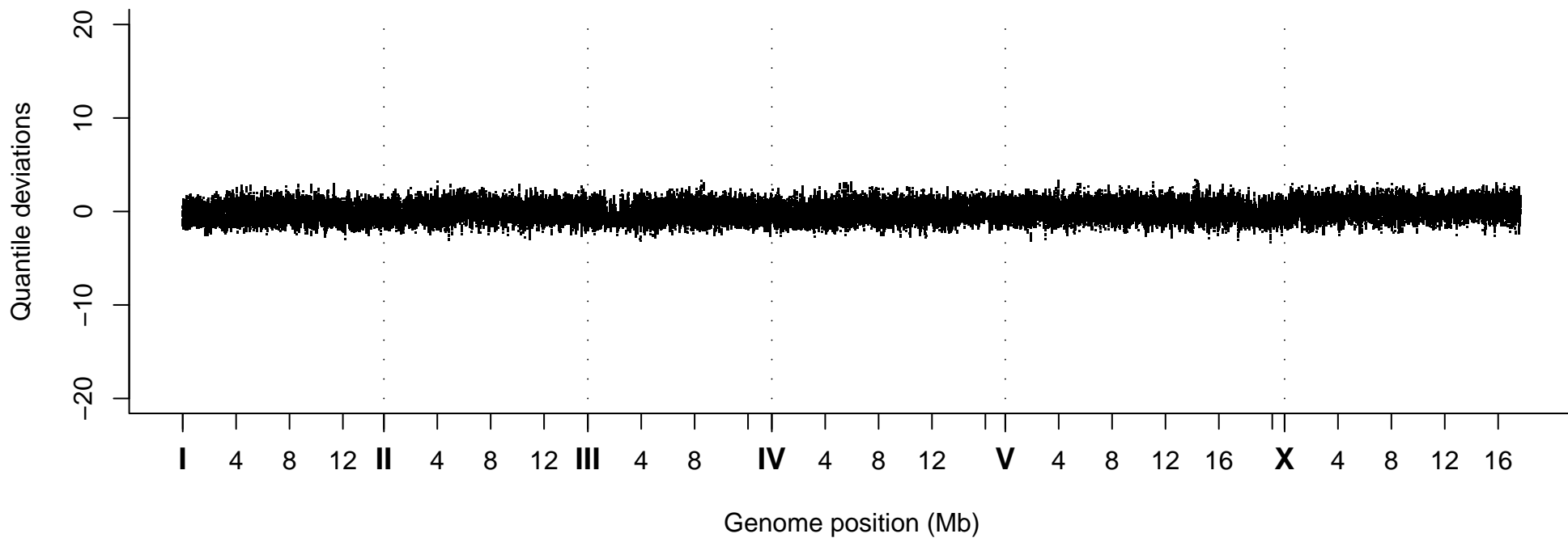
Quantile Deviations, Strain VC40975
