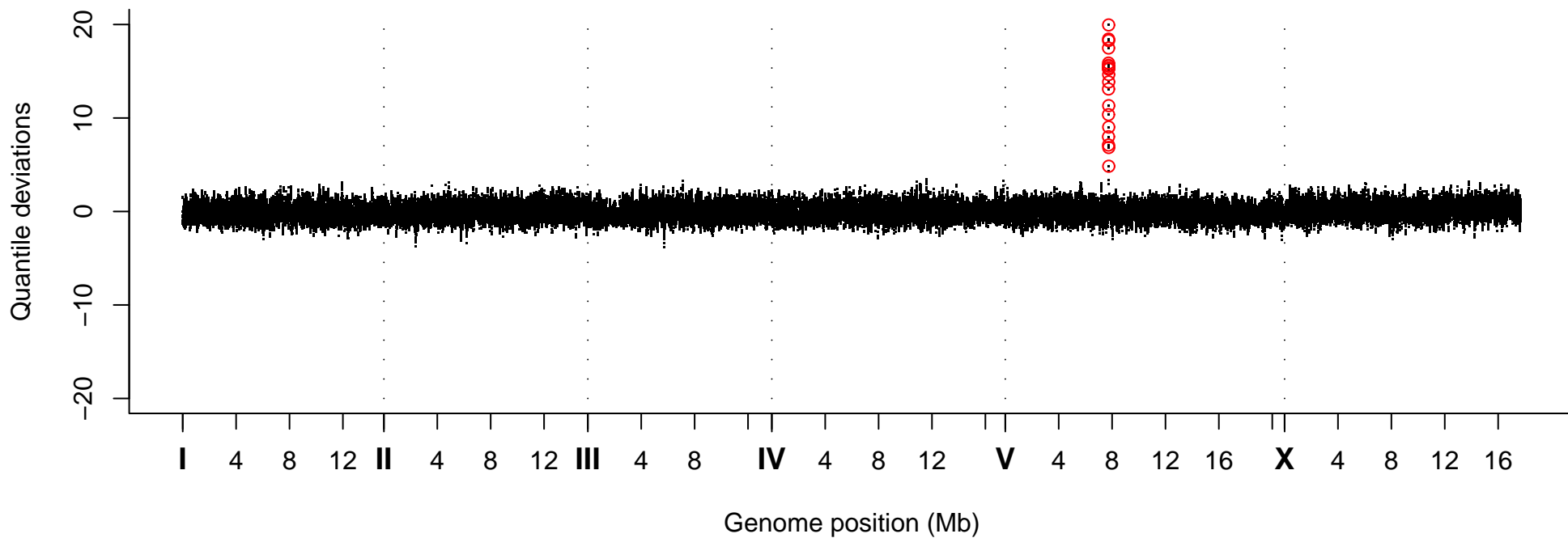
Quantile Deviations, Strain VC40978
