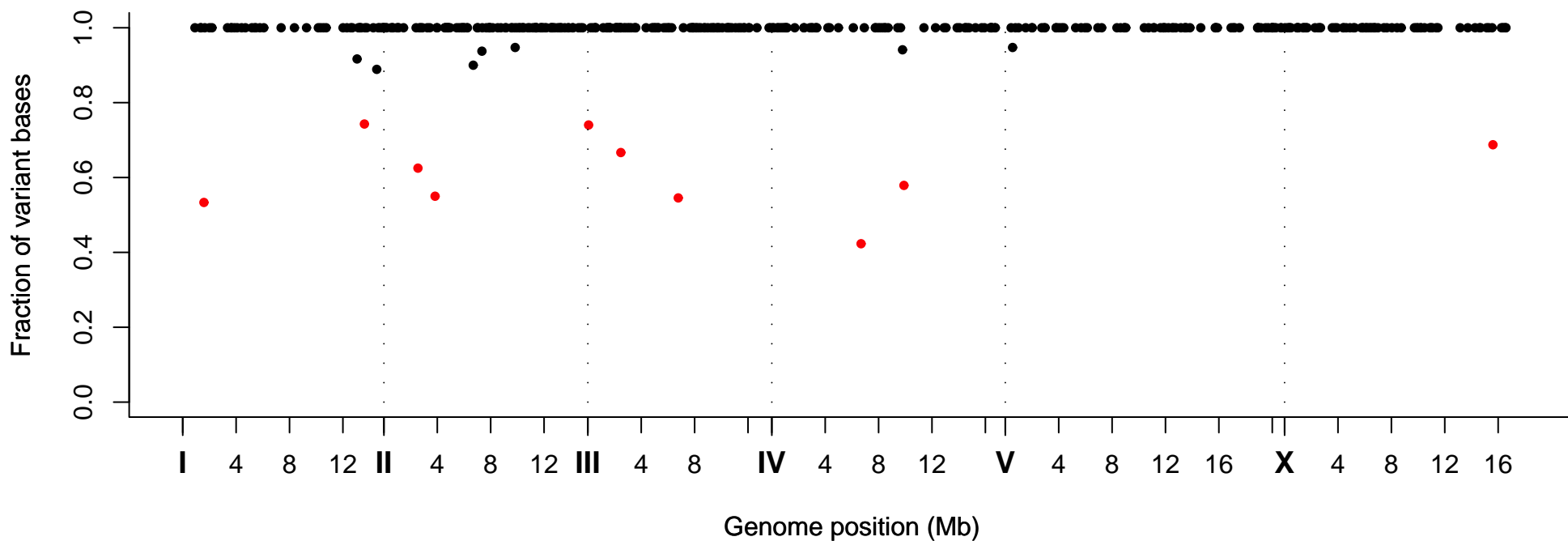
Fraction of Variant Bases at Position, Strain VC40978
