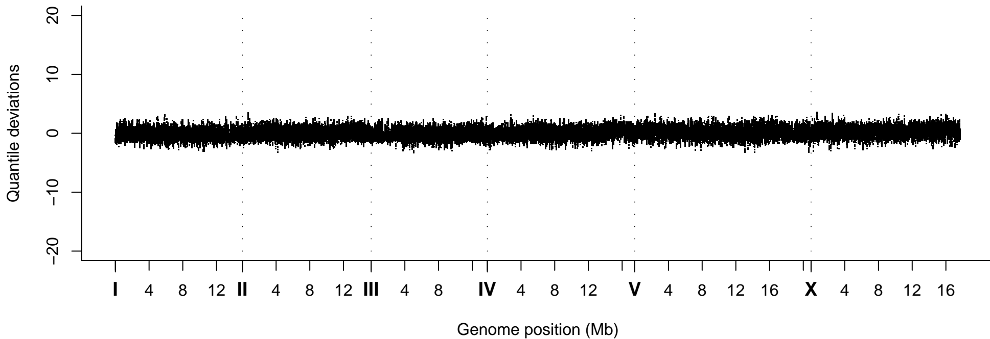
Quantile Deviations, Strain VC40979
