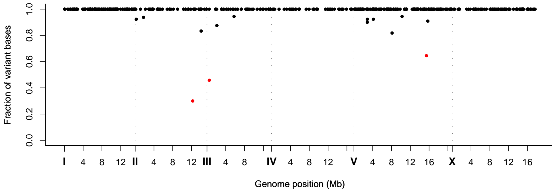
Fraction of Variant Bases at Position, Strain VC40979
