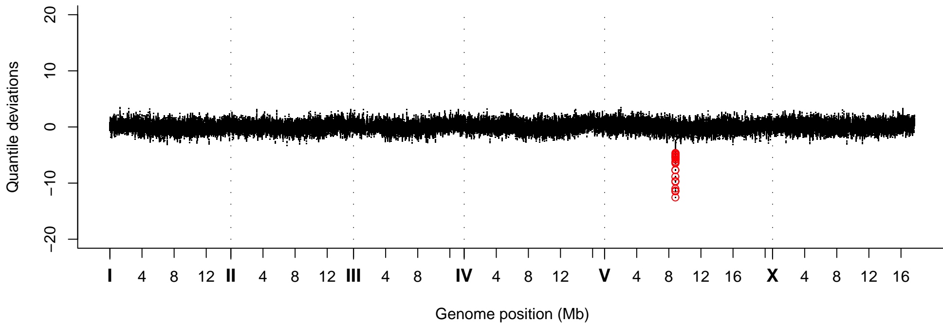
Quantile Deviations, Strain VC40986
