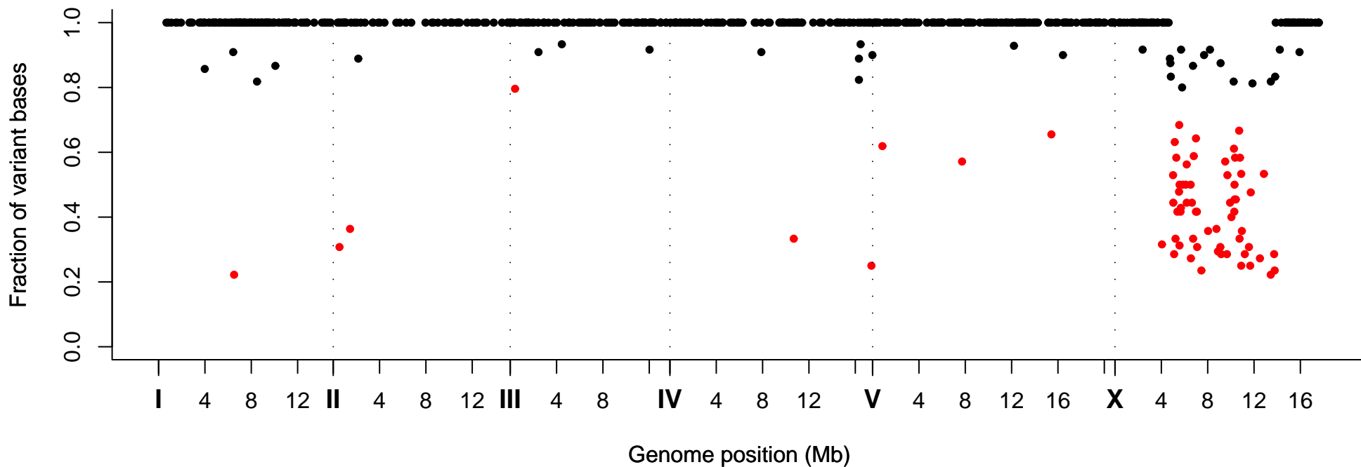
Fraction of Variant Bases at Position, Strain VC40986
