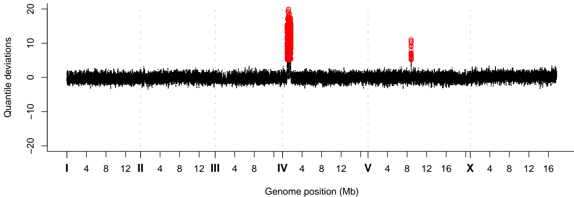
Quantile Deviations, Strain VC40991
