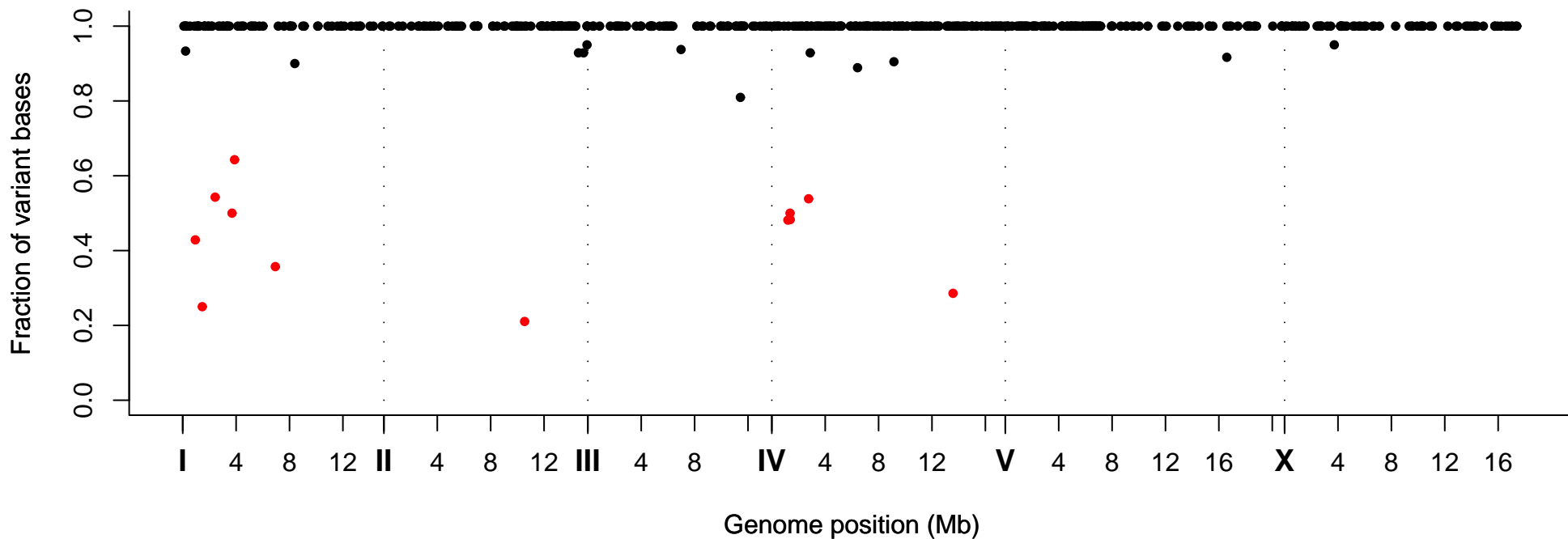
Fraction of Variant Bases at Position, Strain VC40991
