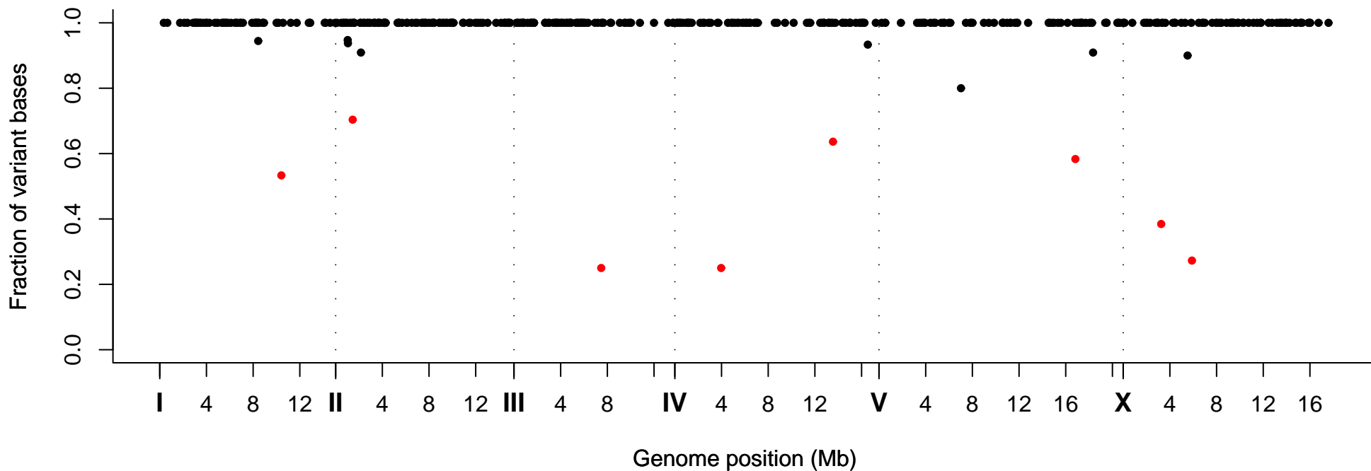
Fraction of Variant Bases at Position, Strain VC40992
