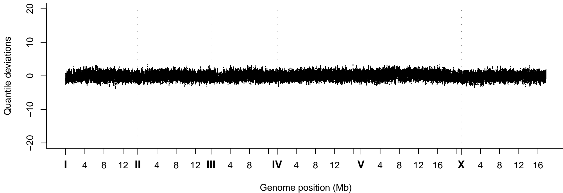
Quantile Deviations, Strain VC40992
