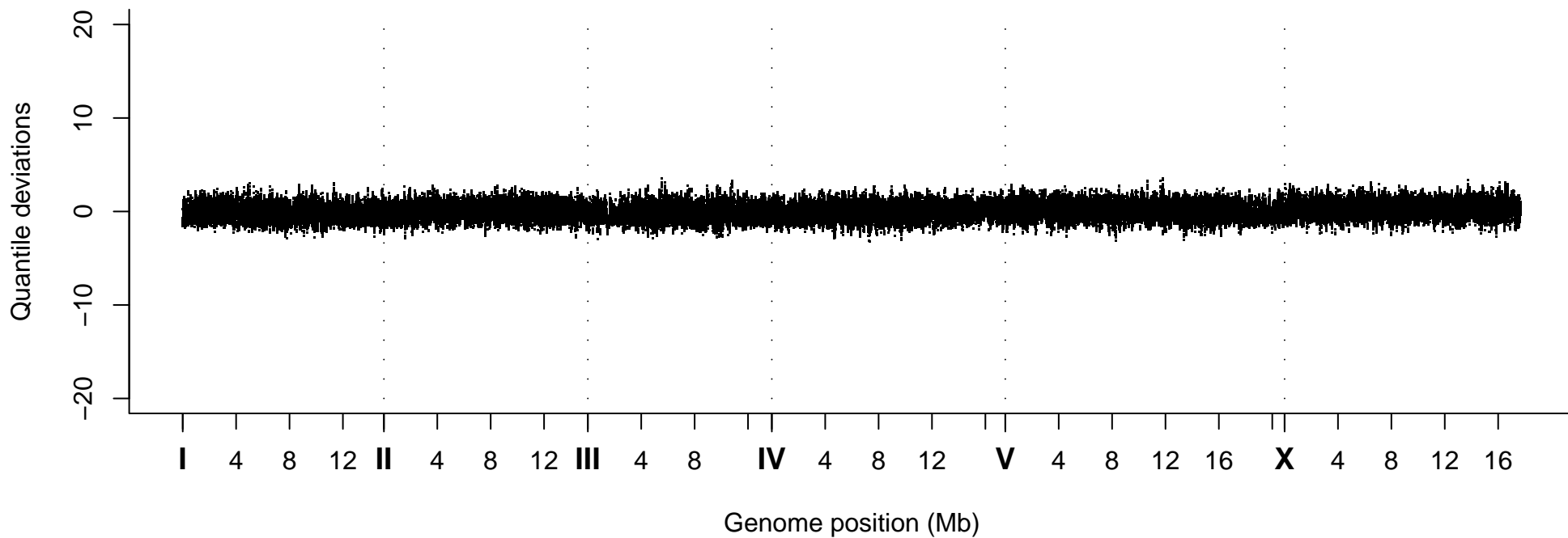
Quantile Deviations, Strain VC40993
