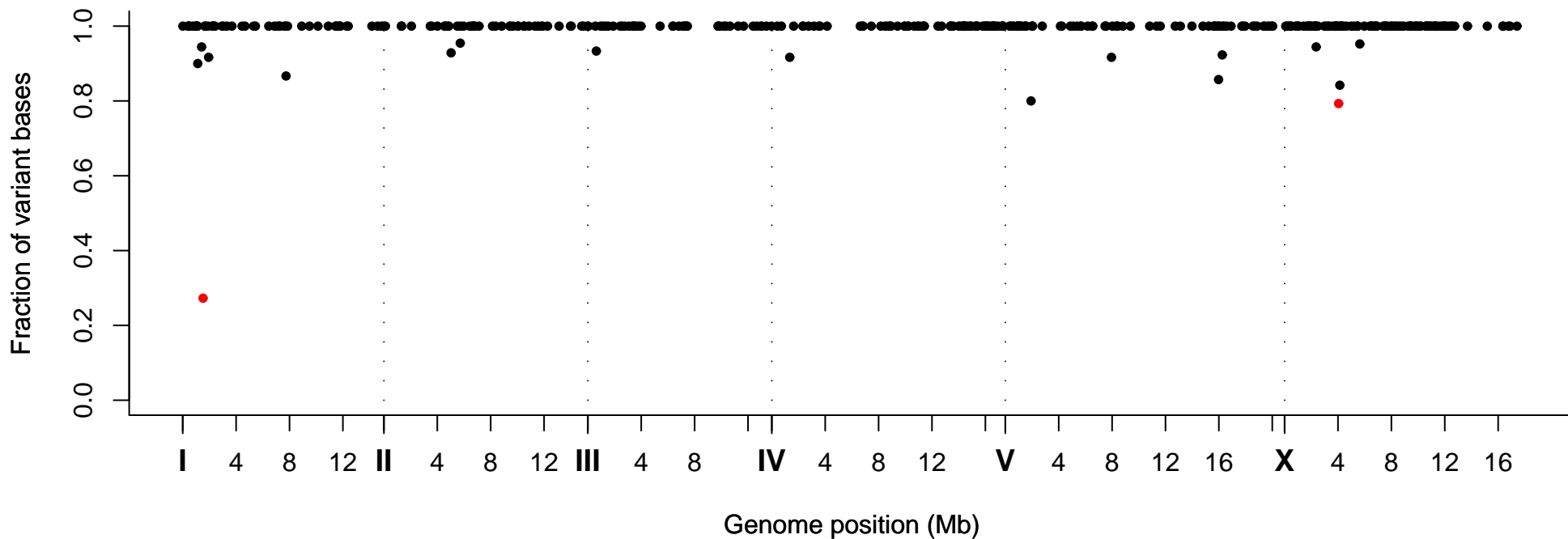
Fraction of Variant Bases at Position, Strain VC40993
