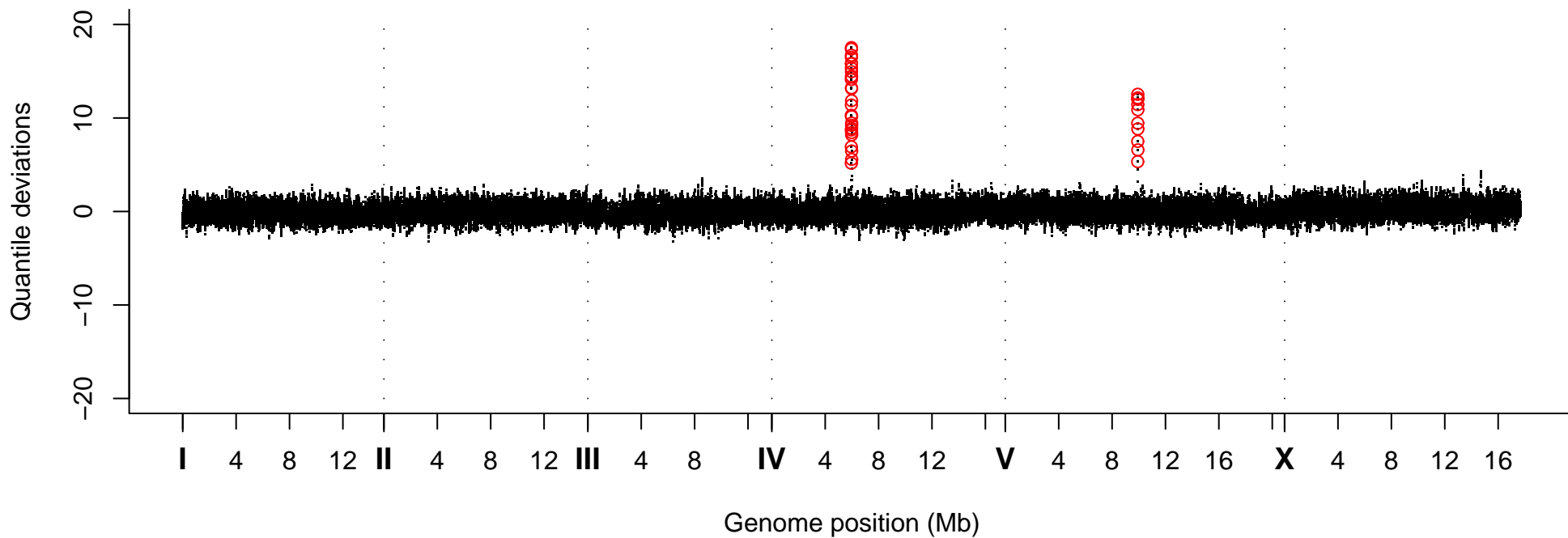
Quantile Deviations, Strain VC41006
