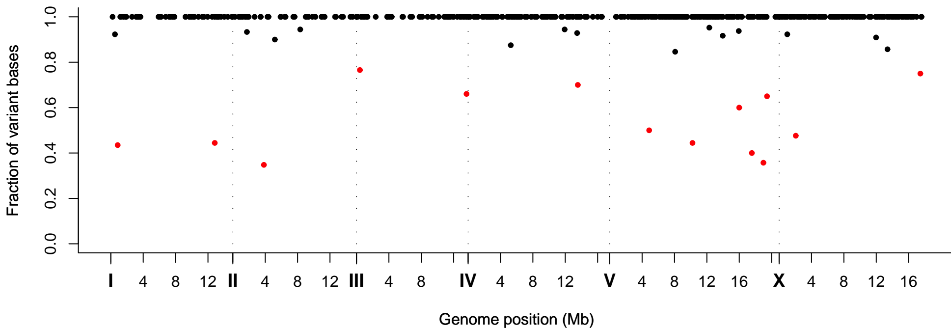
Fraction of Variant Bases at Position, Strain VC41006
