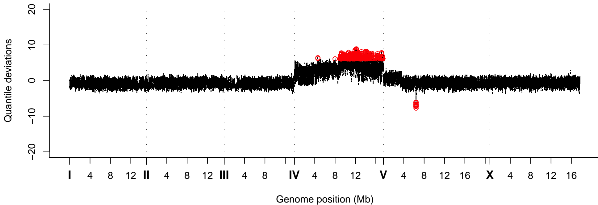
Quantile Deviations, Strain VC41010
