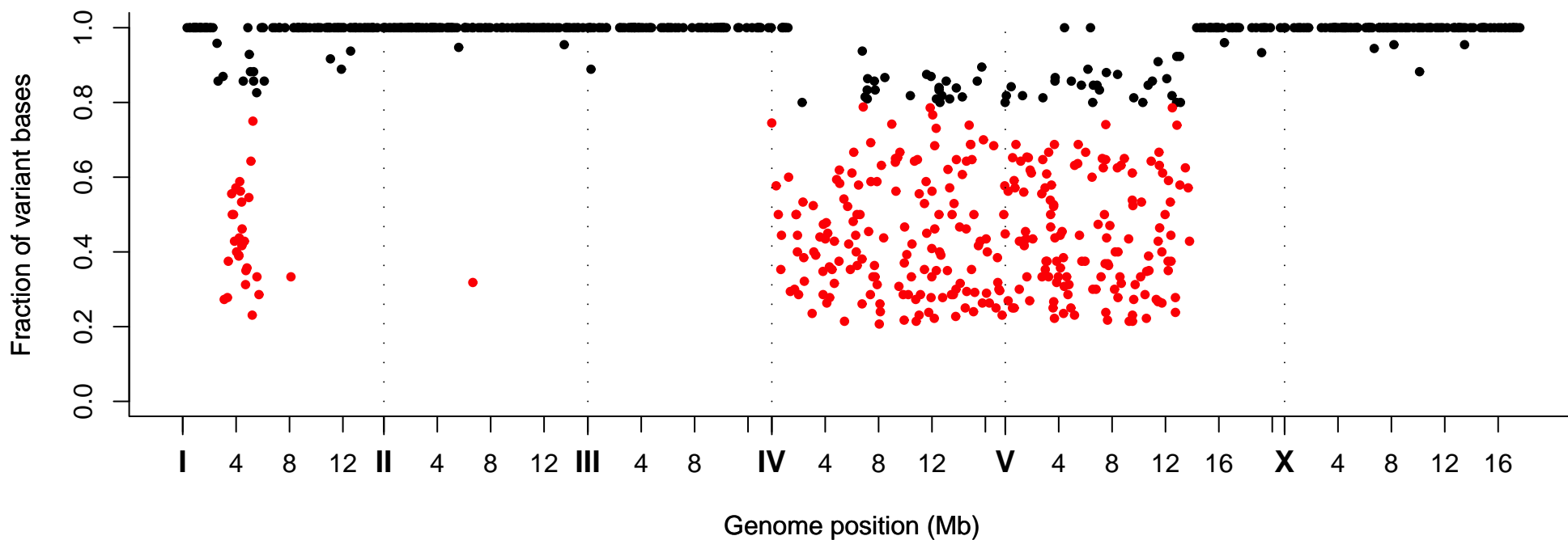
Fraction of Variant Bases at Position, Strain VC41010
