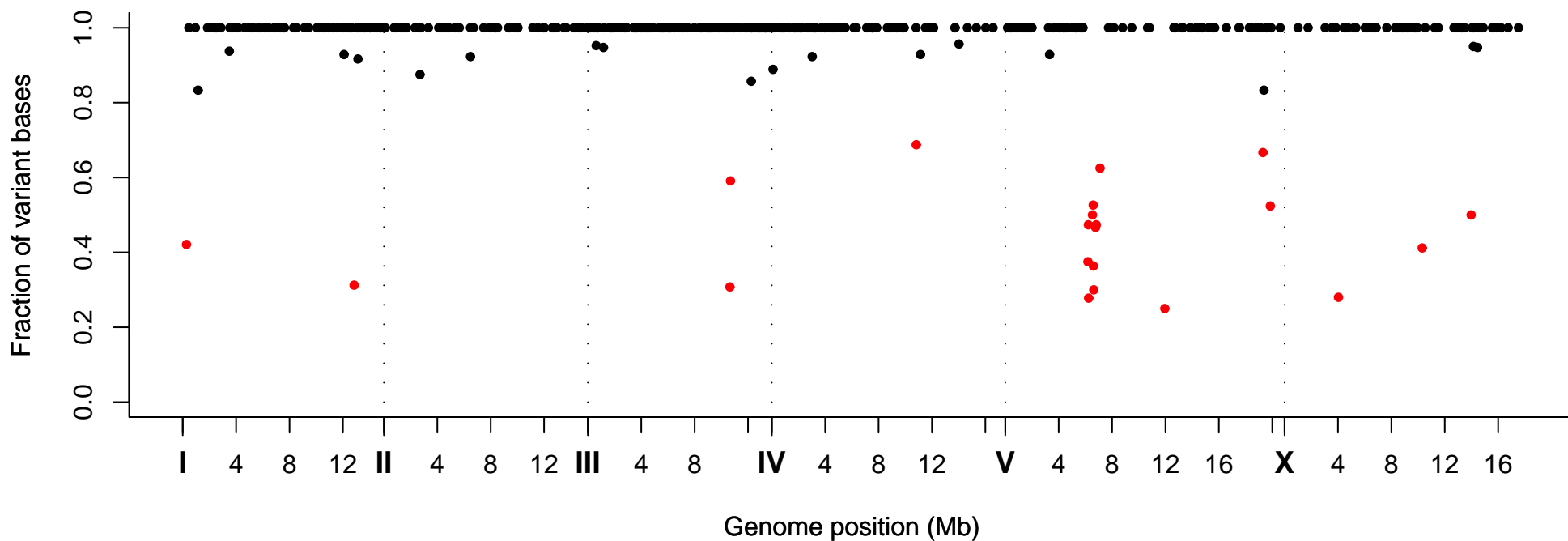
Fraction of Variant Bases at Position, Strain VC41024
