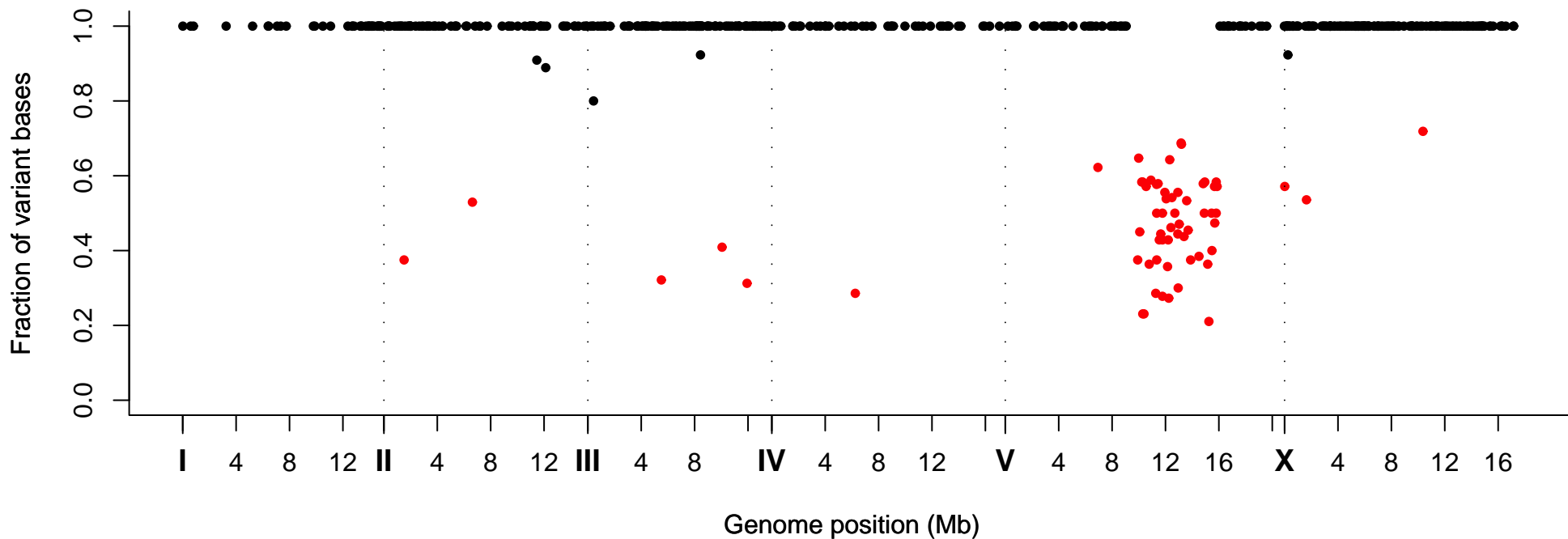
Fraction of Variant Bases at Position, Strain VC41026
