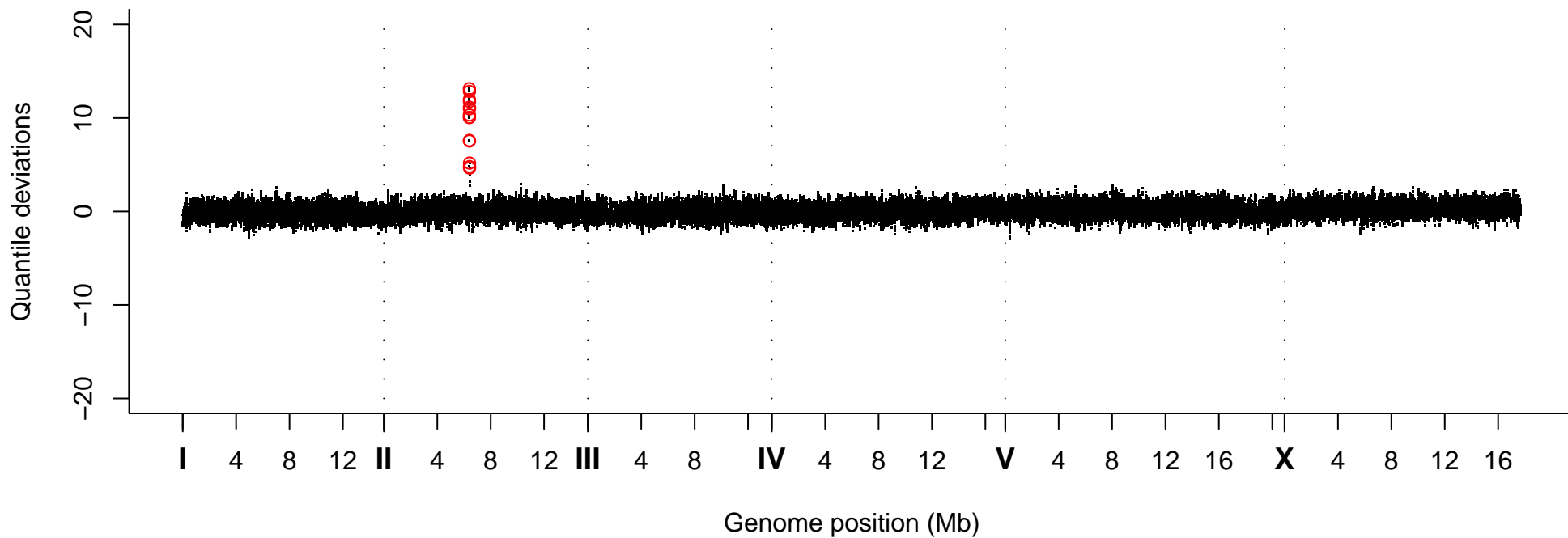
Quantile Deviations, Strain VC41026
